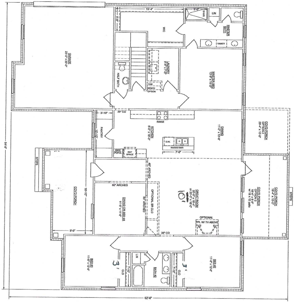
FLOOR PLAN W/ OPTIONS SCALE 1/4" = 1'-0"
