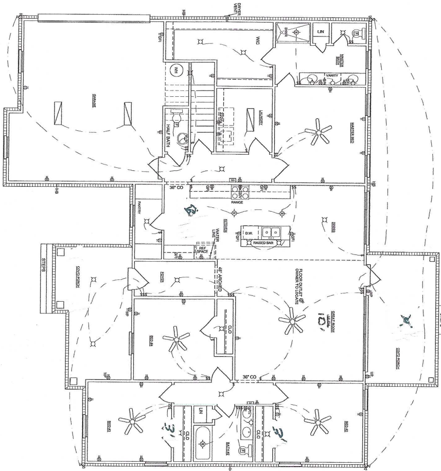
ELECTRICAL PLAN SCALE 1/4" = 1'-0"
