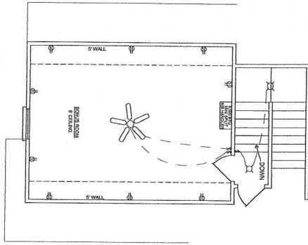
ELECTRICAL PLAN SCALE 1/4" = 1'-0"
