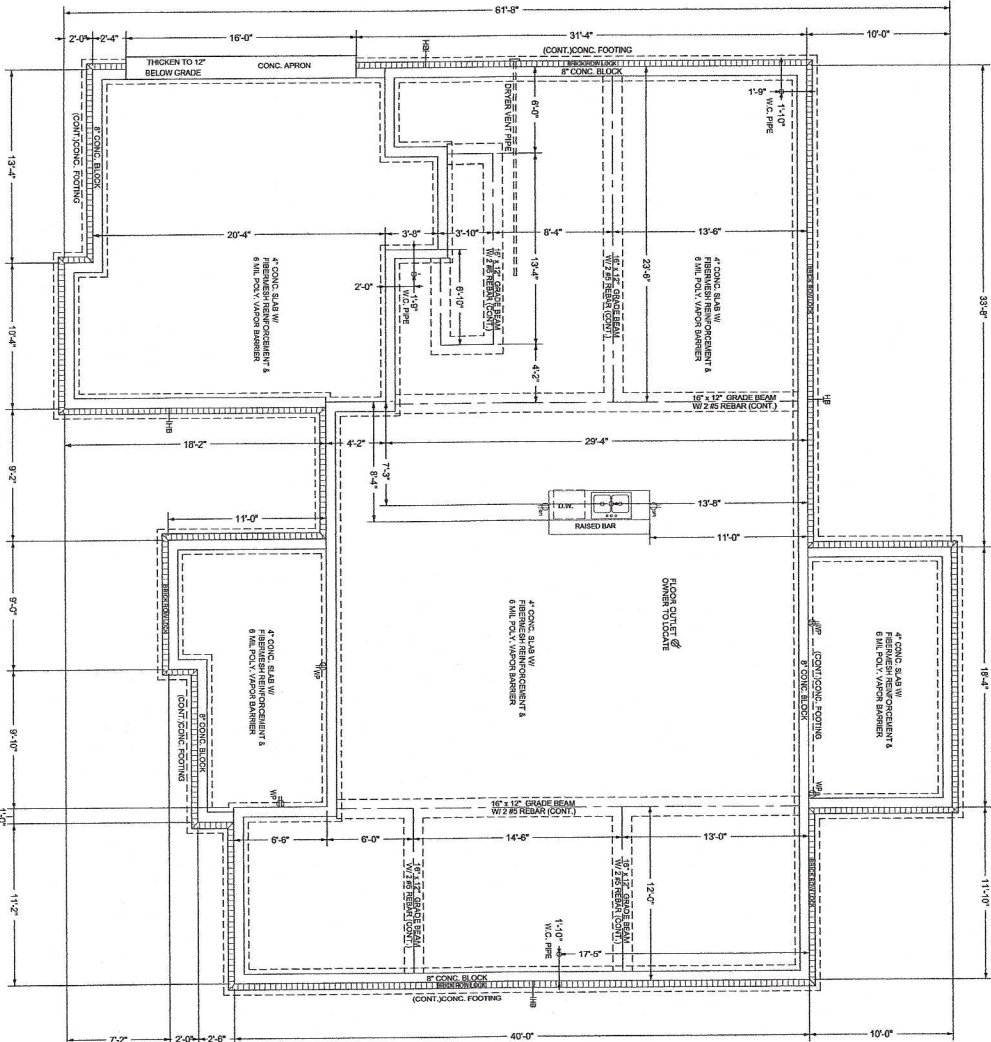
FOUNDATION PLAN SCALE: 1/4\"/>
