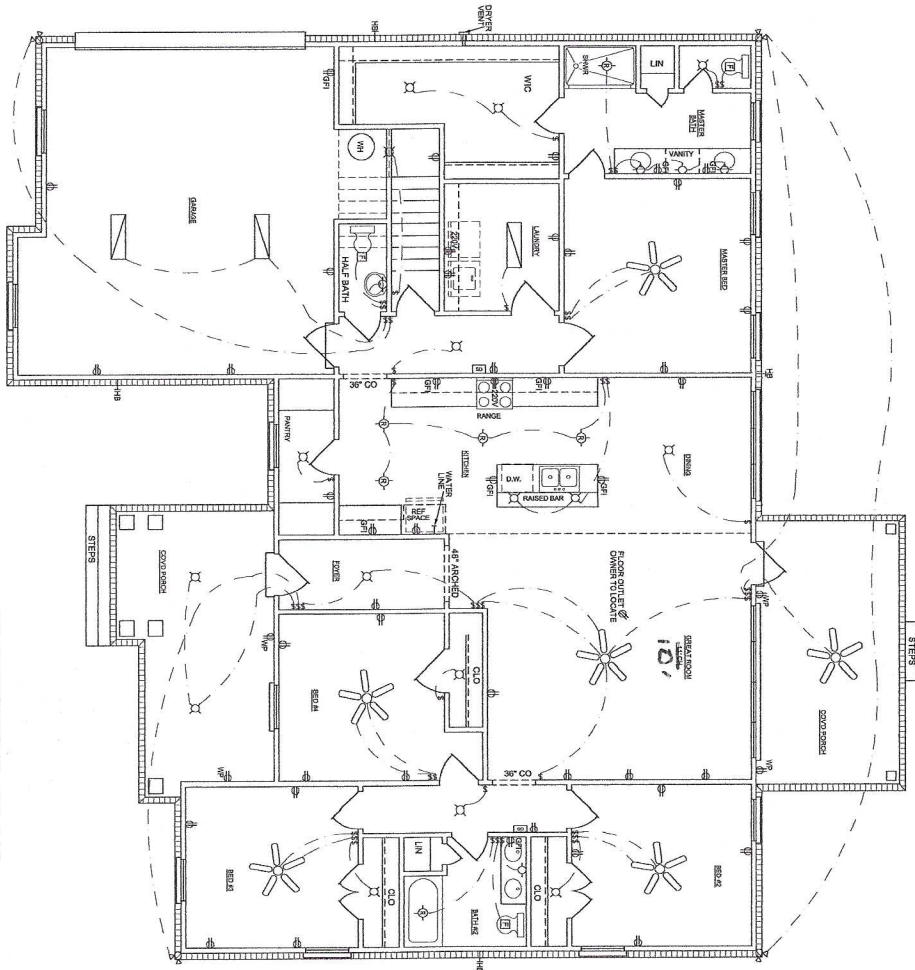
ELECTRICAL PLAN SCALE 1/4" = 1'-0"
